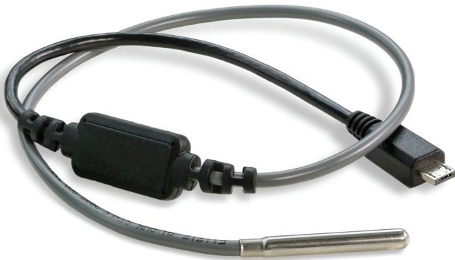
Model BFA10094 Temperature Probe with AP300 Connector for connection to Accessory Pack input
