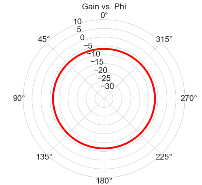
Gain dBi, Conical Cut \Theta = 45 , Frequency 1799.60(MHz)
