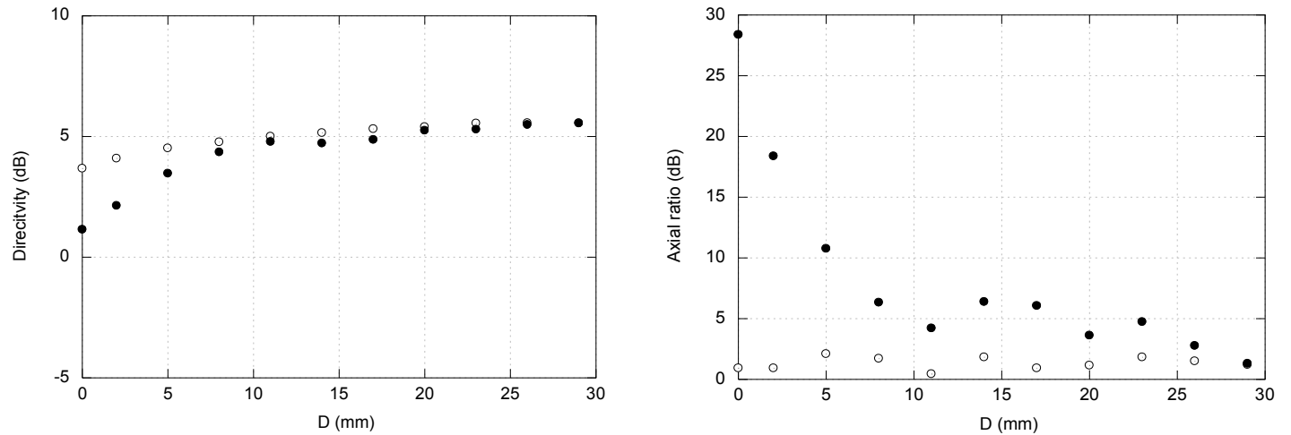
Figure 9 - (a) Directivity and (b) axial ratio at 1576 MHz a function of the distance d from the center of the ground plane. Legend: white dots: directivity/axial ratio at center frequencies; black dots: directivity/axial ratio at 1576 MHz.
