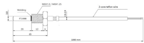
PROBE PT1000
