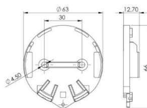
PUCK HOLDER
